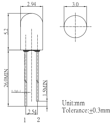
LED Outline Dimension
