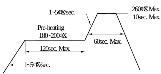
< 2 : Lead-free Solder >
