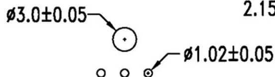
PCB Layout
