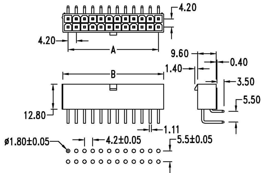
P. C. B . hole dimensions
