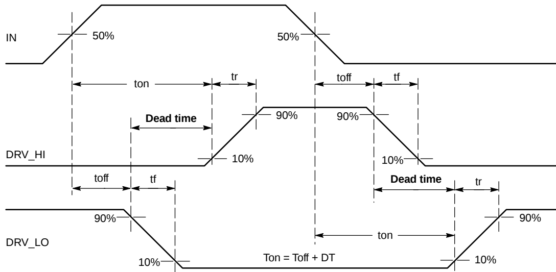
Figure 5. Timing Definitions
