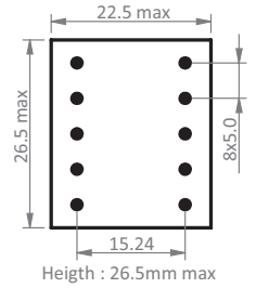
E 25 reinforced insulation creepage distances: 8mm
