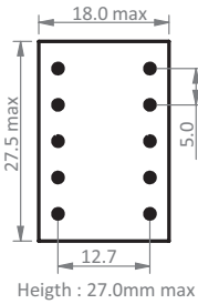
EF 25 reinforced insulation creepage distances: 6mm
