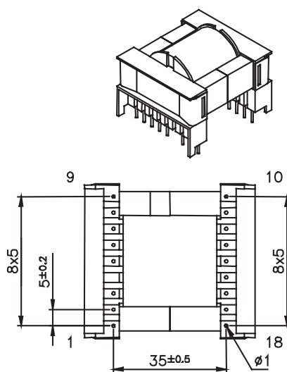
Bottom View (Pin side)
