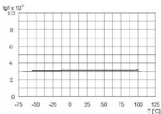
tgδ-T
