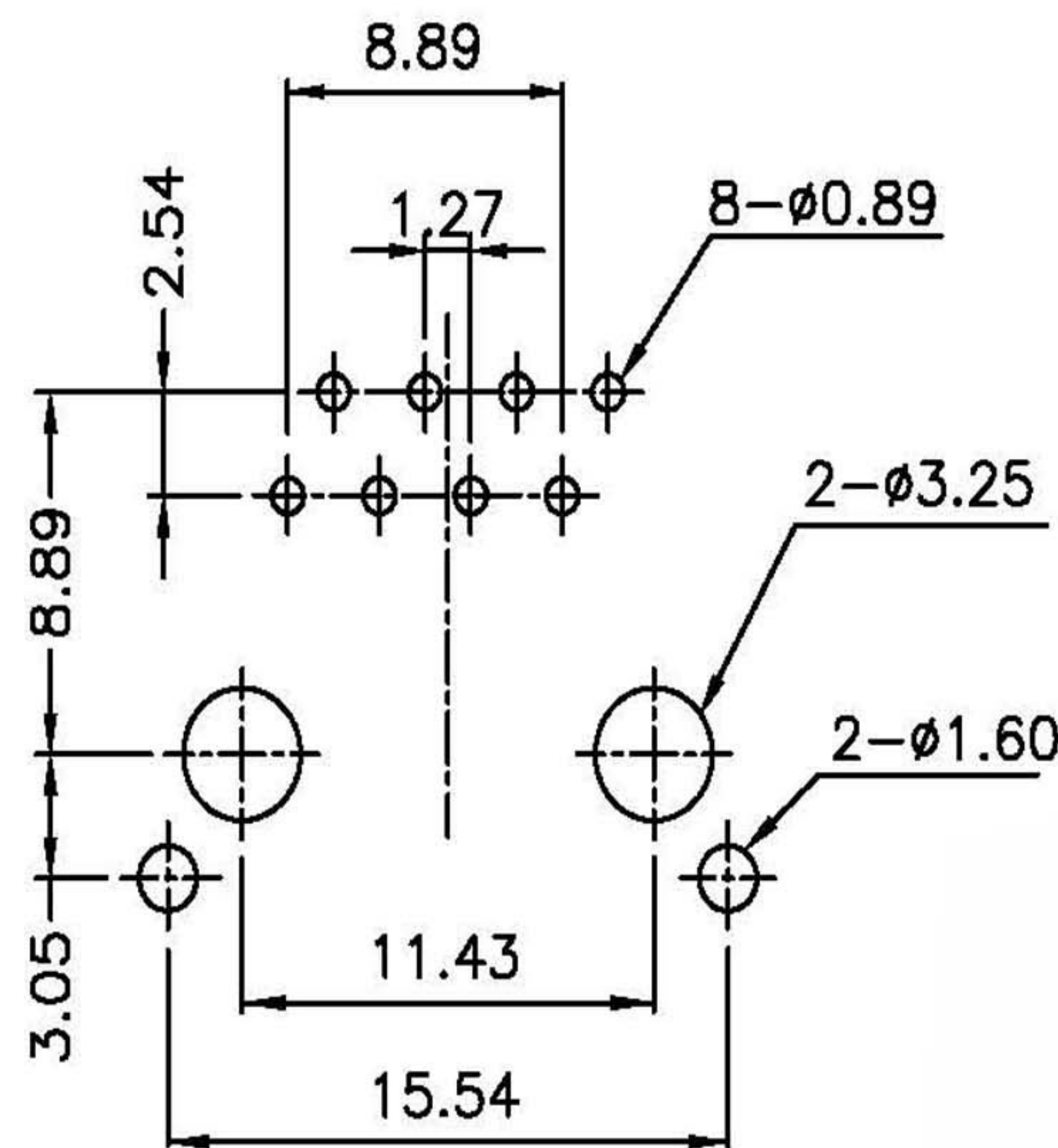
PC BOARD LAYOUT
