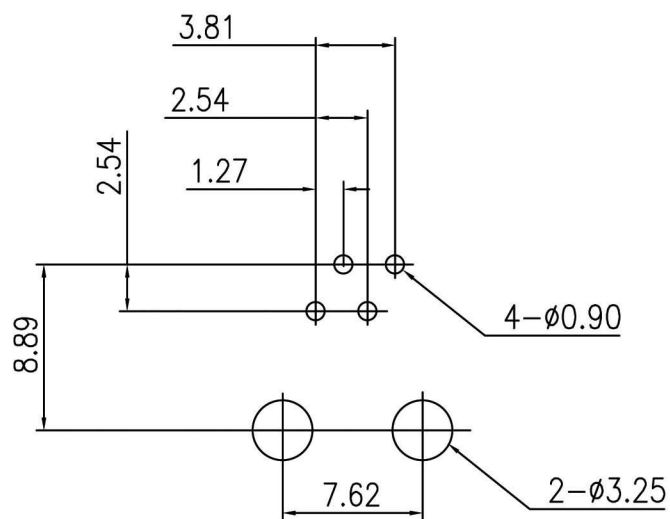
PCB Layout
