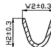
Section "B-B" 4/1
