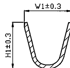
Section "C-C" 4/1
