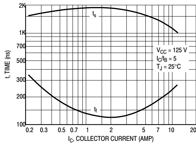
Figure 12. Turn-Off Time
