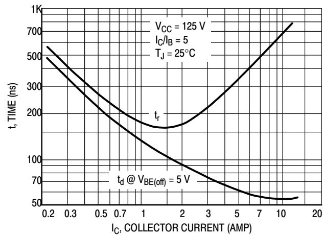
Figure 11. Turn-On Time
