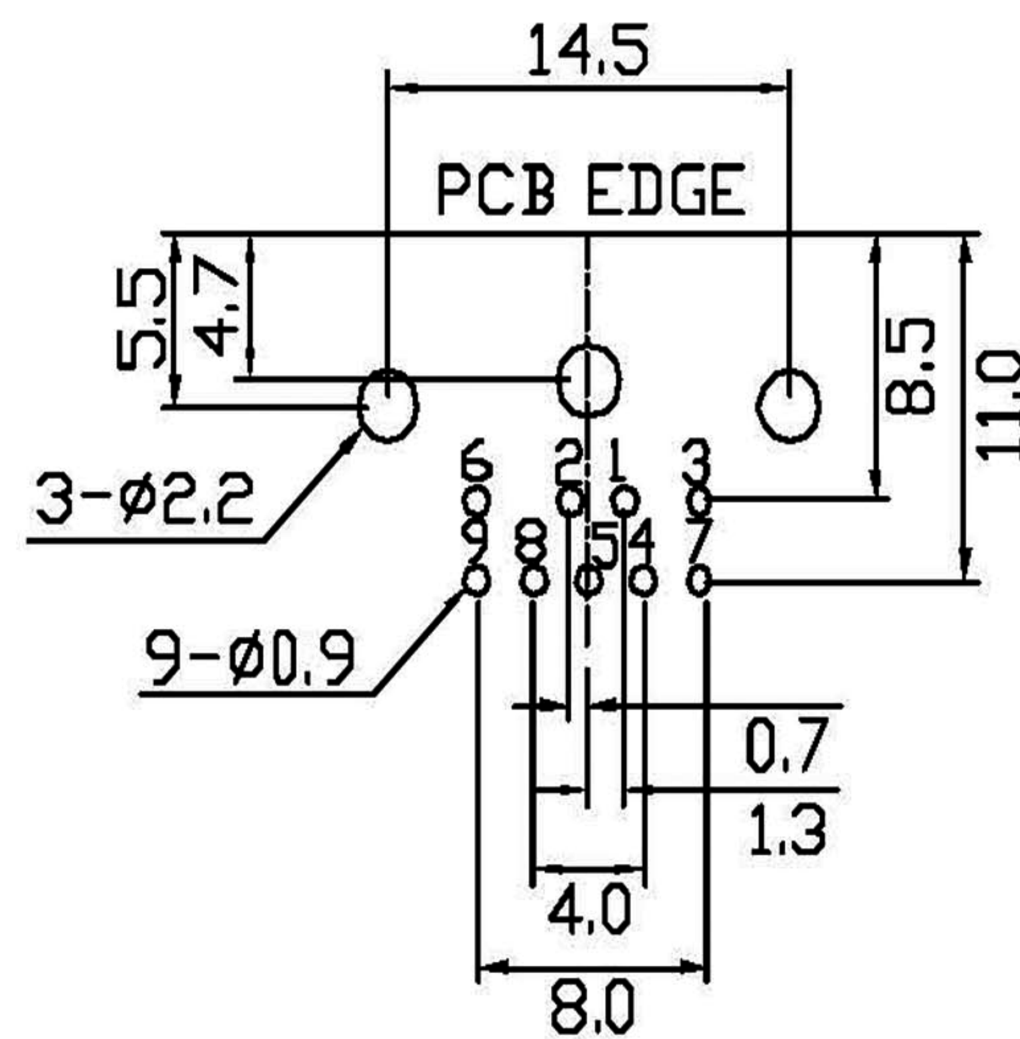
PCB LAYOUT (BOTTOM VIEW)
