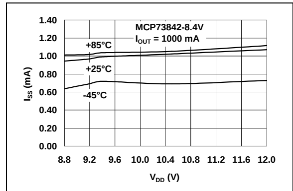
FIGURE 2-11: Supply Current ( I_{SS} ) vs. Supply Voltage ( V_{DD} ).
