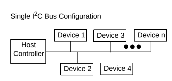
FIGURE 5-1: Typical Application I 2 C Bus Configurations.
