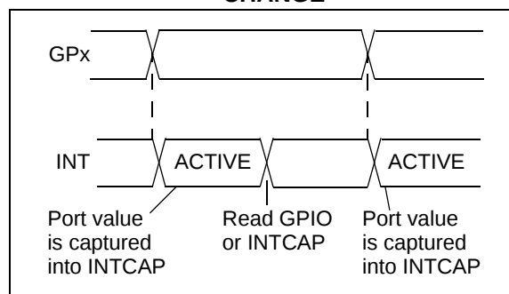
FIGURE 1-11: INTERRUPT-ON-PIN-CHANGE
