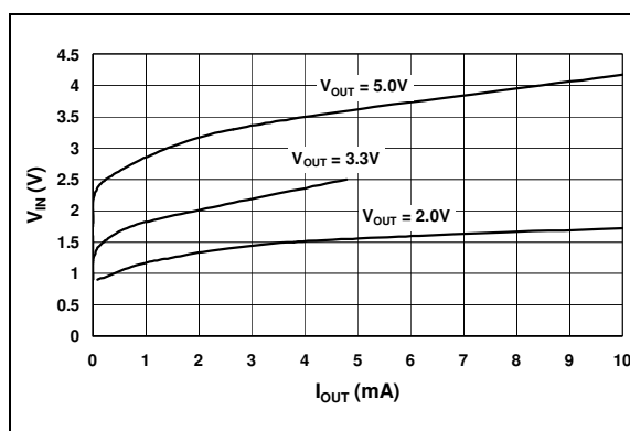
FIGURE 2-12: PWM Pulse Skipping Mode Threshold vs. I_{OUT} .
