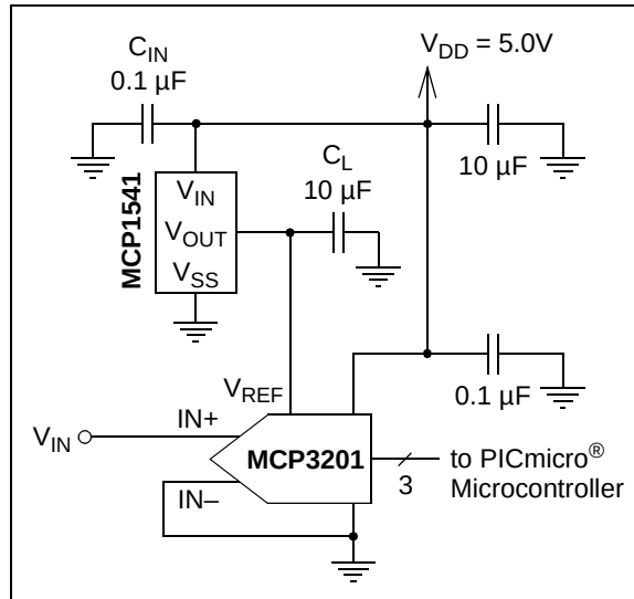
FIGURE 4-4: ADC Reference Circuit.
