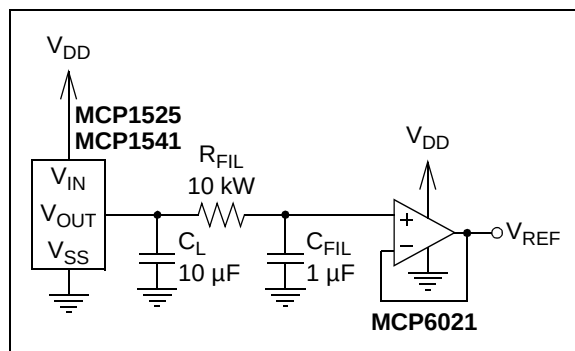
FIGURE 4-2: Output Noise-Reducing Filter.
