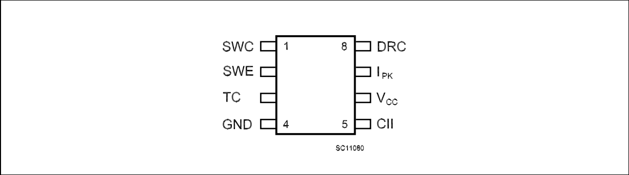
Figure 2. Pin connections
