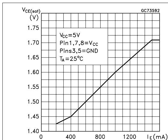
Figure 3. Emitter follower configuration output saturation voltage vs emitter current
