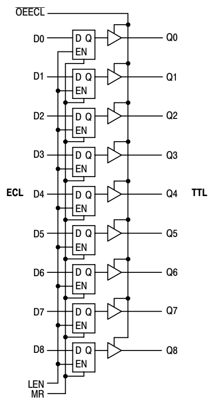
Figure 2. Logic Diagram
