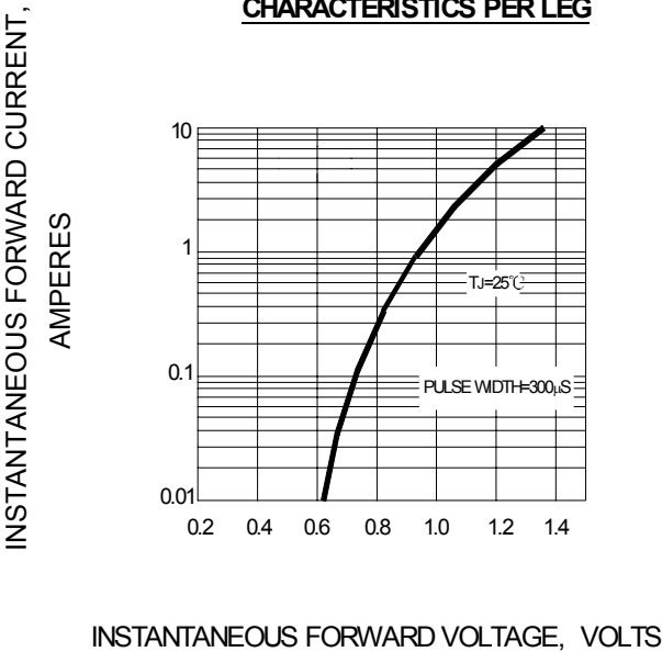
FIG.3 – TYPICAL FORWARD VOLTAGE CHARACTERISTICS PER LEG
