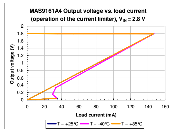
Figure 11. MAS9161A4 output voltage vs. load current (operation of the current limiter). V_{IN} = 2.8 \text{ V} .
