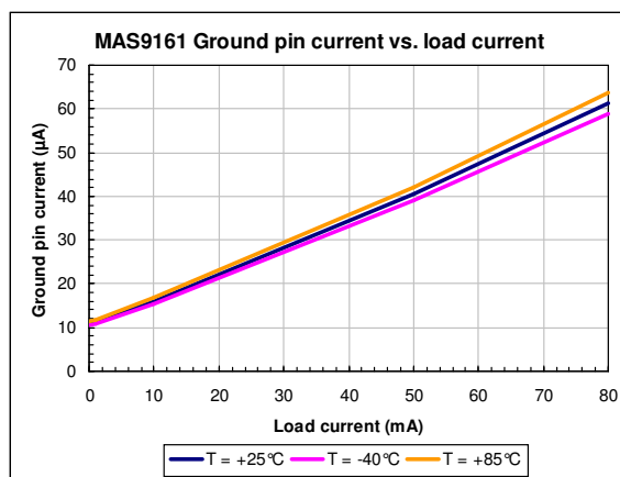
Figure 12. Ground pin current vs. load current.
