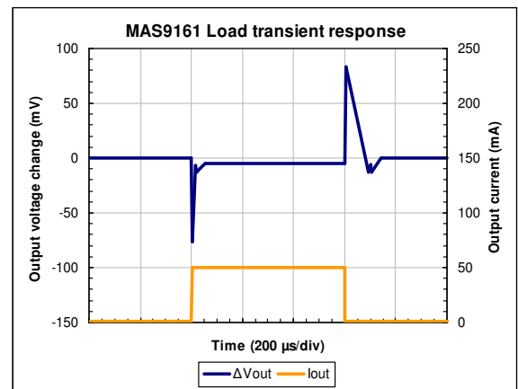
Figure 7. Load transient response. I_{OUT} = 1\text{...}50\text{ mA} in 2\text{ }\mu\text{s} .
