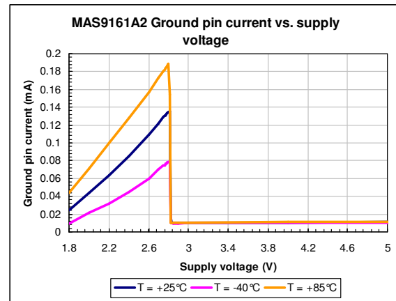
Figure 9. MAS9161A2 ground pin current against the supply voltage. I_{OUT} = 0 \text{ mA} .
