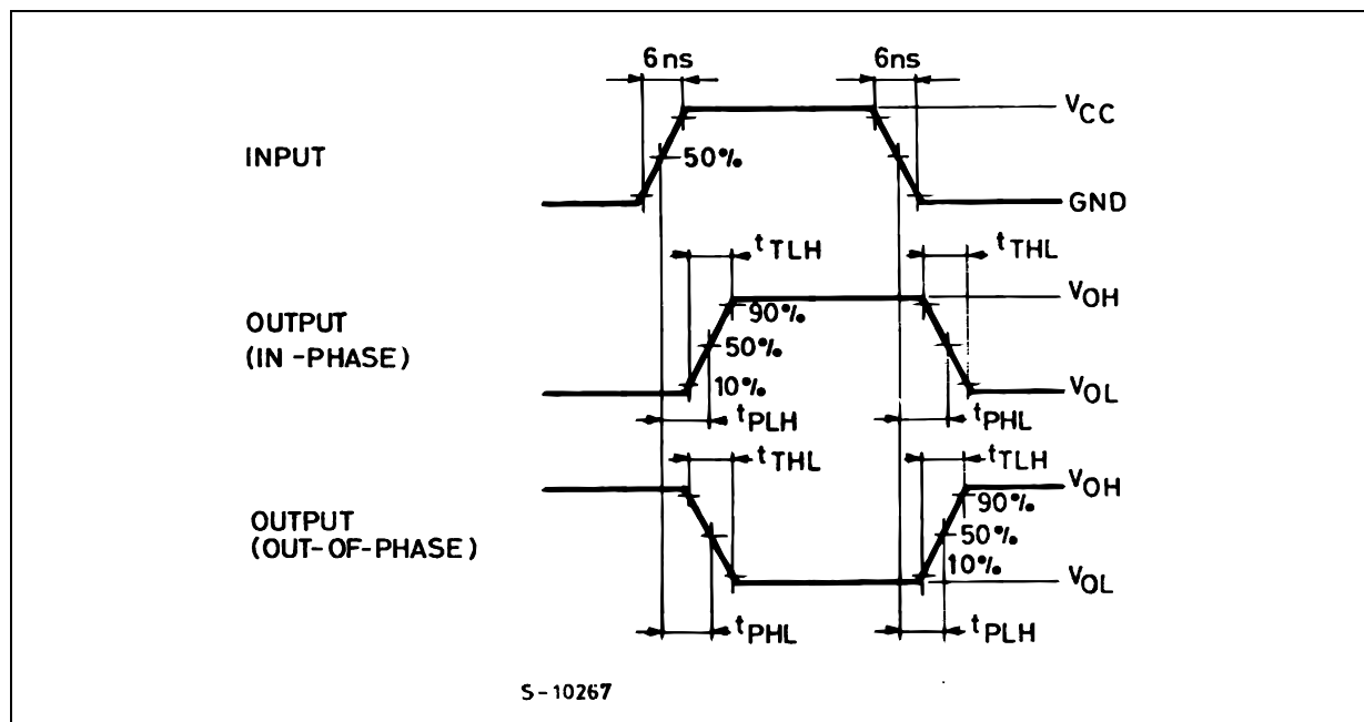
WAVEFORM 1: PROPAGATION DELAY TIMES ( f=1\text{MHz} ; 50% duty cycle)
