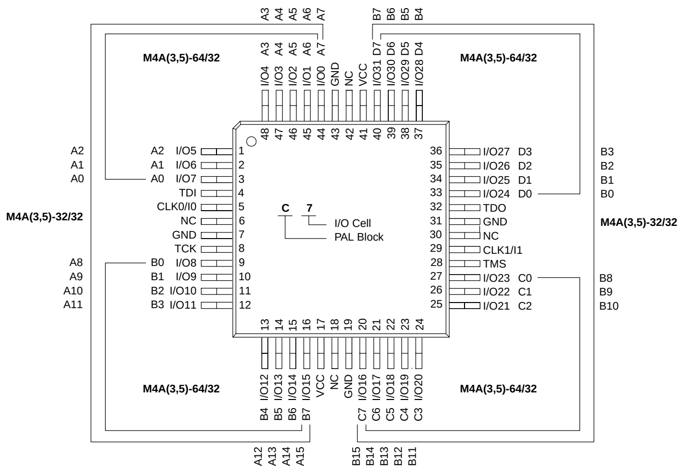
48-Pin TQFP
