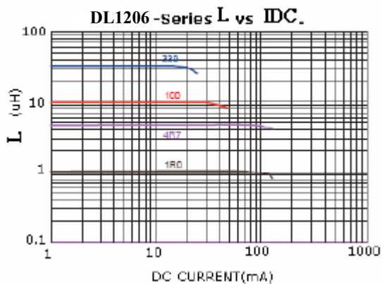
Inductance-Current Characteristics
