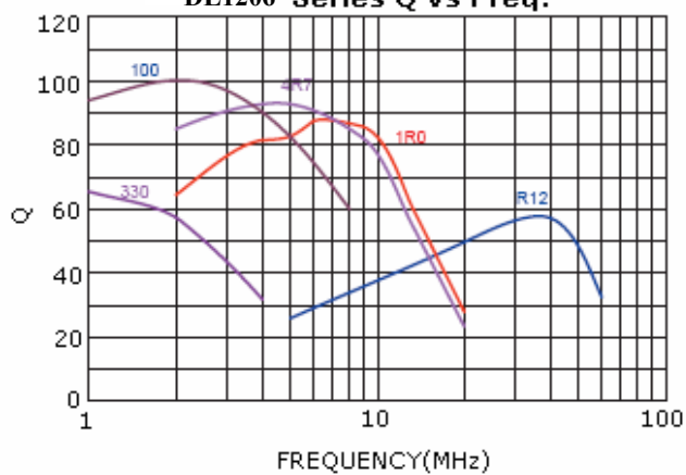
DL1206-Series Q vs Freq.
