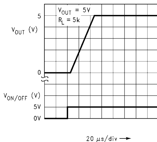
Turn-On Waveform
