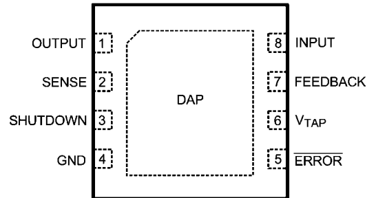
8-Lead LLP
