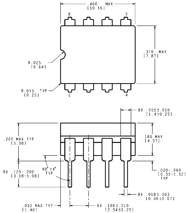
Ceramic Dual-In-Line Package (J) NS Package Number J08A
