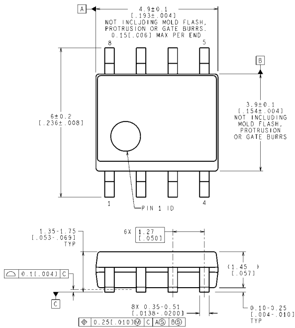
Surface Mount Package (M) NS Package Number M08A
