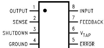
Dual-In-Line Packages (N, J) Surface-Mount Package (M, MM)
