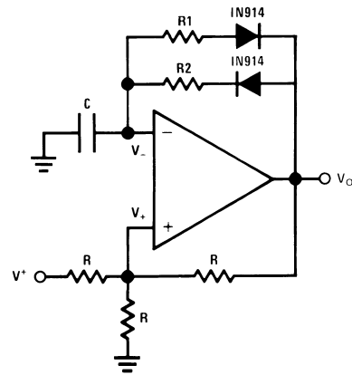
FIGURE 16. Pulse Generator
