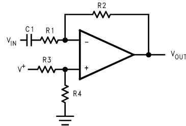
FIGURE 10. Single-Supply Inverting Amplifier
