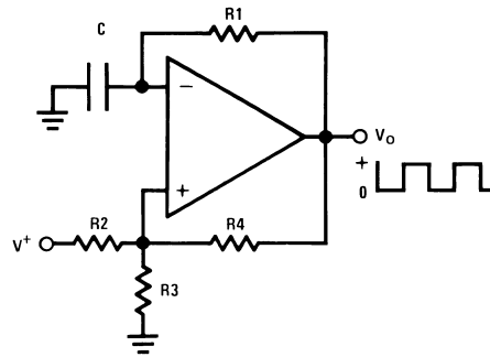
FIGURE 19. Squarewave Generator
