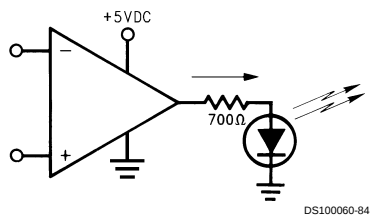
FIGURE 23. LED Driver
