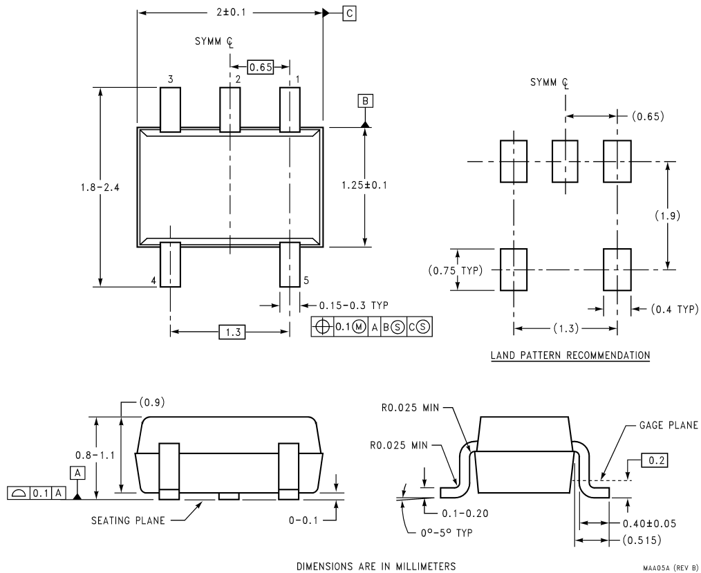
DIMENSIONS ARE IN MILLIMETERS 5-Pin SC70-5 Tape and Reel Order Number LMV321M7 and LMV321M7X NS Package Number MAA05A
