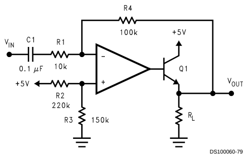
FIGURE 22. Power Amplifier
