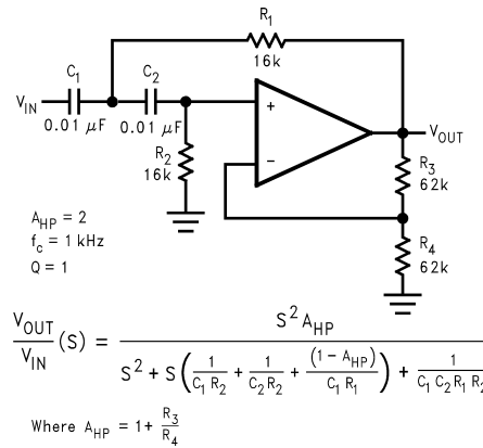
FIGURE 14. Sallen-Key 2nd-Order Active High-Pass Filter
