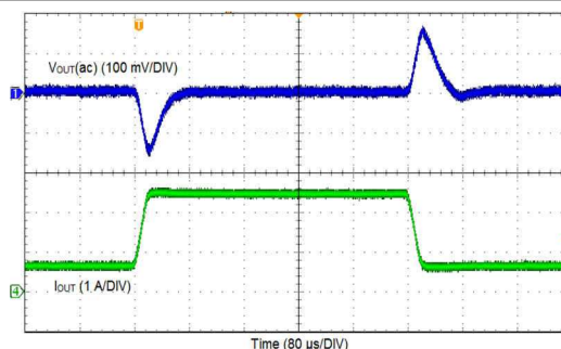
Figure 8-5. DCM Mode
