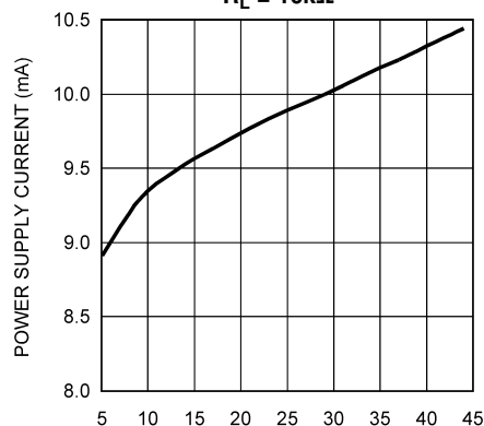
Power Supply Current vs Total Power Supply Voltage R_L = 10k\Omega
