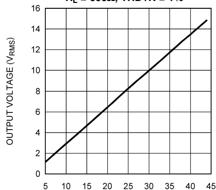
Output Voltage vs Total Power Supply Voltage R_L = 600\Omega , THD+N = 1%
