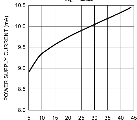
Power Supply Current vs Total Power Supply Voltage R_L = 2k\Omega
