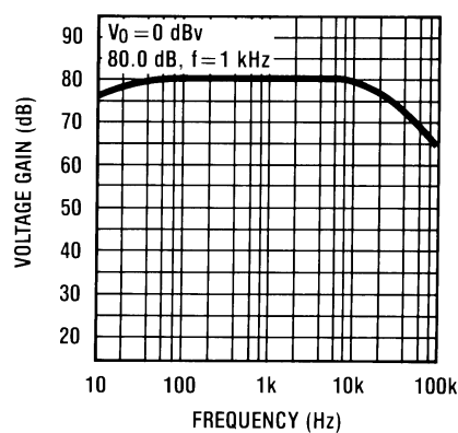
Figure 112. Flat Amp Voltage Gain vs Frequency
