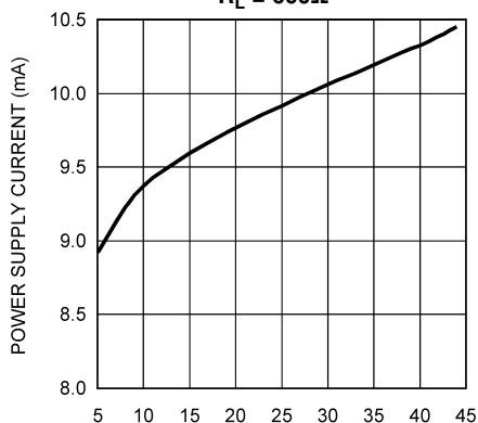
Power Supply Current vs Total Power Supply Voltage R_L = 600\Omega
