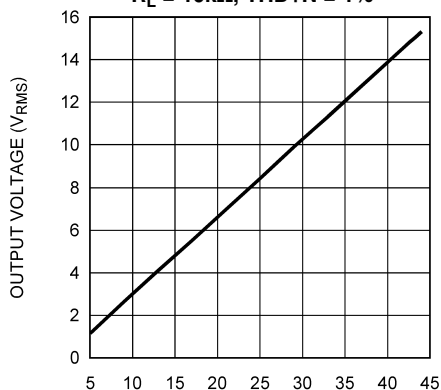
Output Voltage vs Total Power Supply Voltage R_L = 10k\Omega , THD+N = 1%
