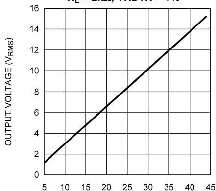
Output Voltage vs Total Power Supply Voltage R_L = 2k\Omega , THD+N = 1%
