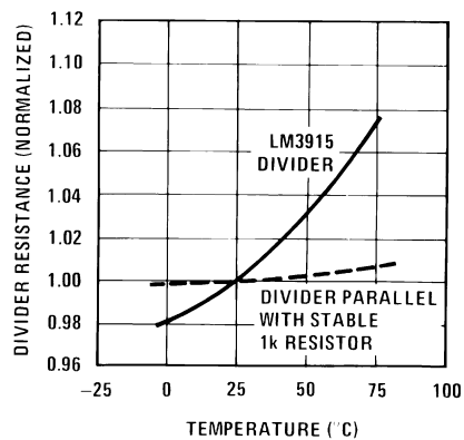
Total Divider Resistance vs Temperature
