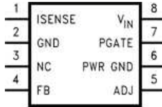
DGK Package 8-Pin VSSOP Top View
