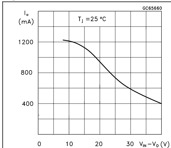
Figure 4. Current limit
