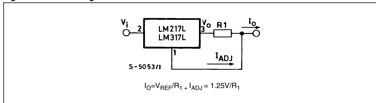
Figure 9. Current regulator
