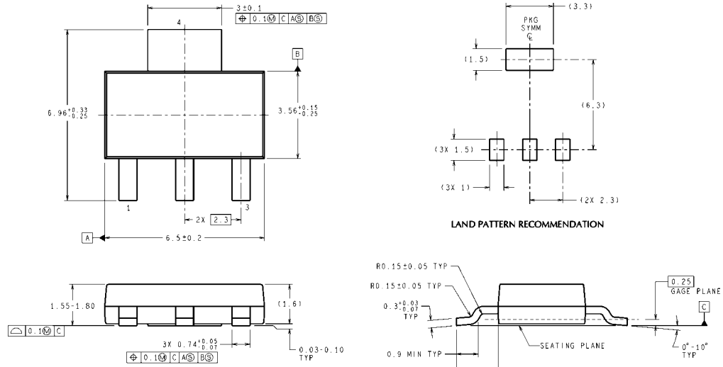
3-Lead SOT-223 Package NS Package Number MP04A
