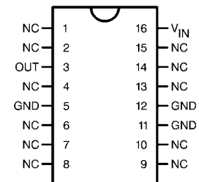
16-Lead Ceramic Surface-Mount Package (WG)
