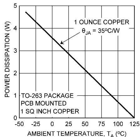
FIGURE 4. Maximum Power Dissipation vs. T_A for the TO-263 Package
