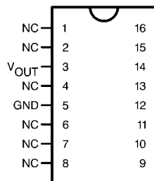
16-Lead Dual-in-Line Package (J)
