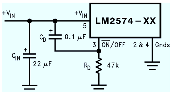
Figure 17. Delayed Start-Up
