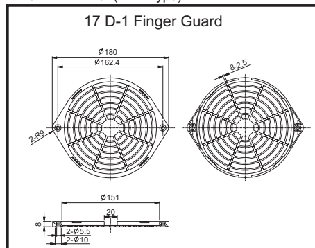
For 172mm Fan(17 D Type)
