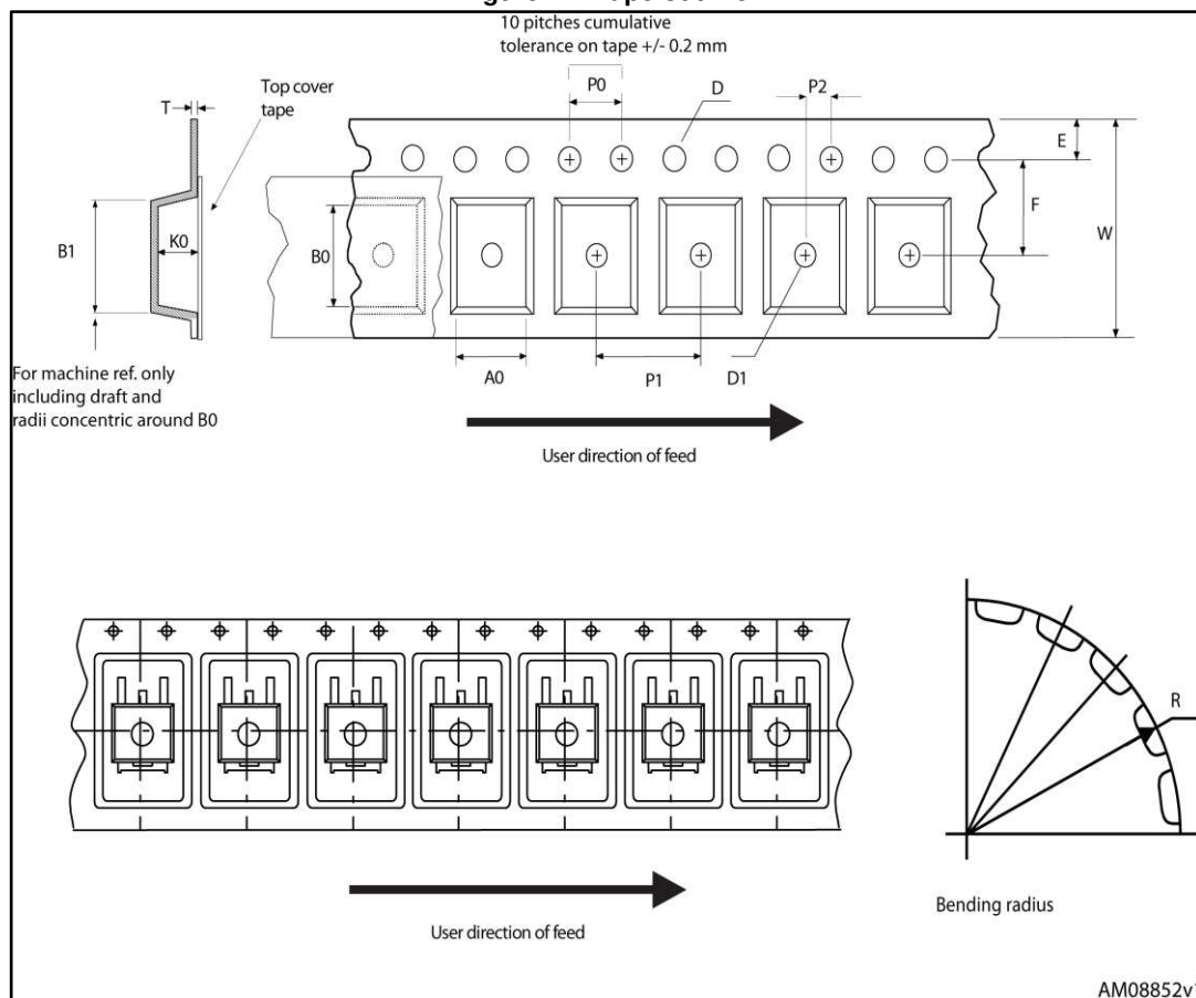
Figure 47: Tape outline
