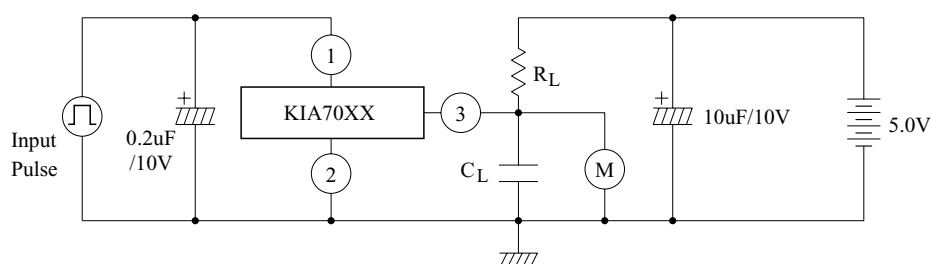
TEST CIRCUIT 2.
