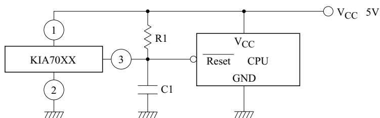
(2) CPU RESETING
