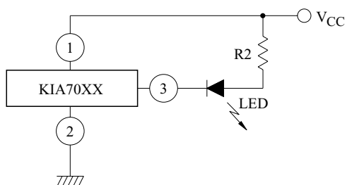
(1) BATTERY LOW INDICATOR
