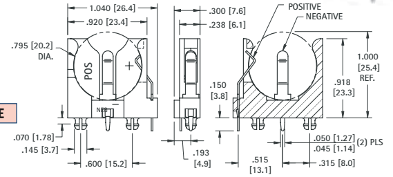
Mounting Detail
