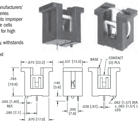
Mounting Detail
