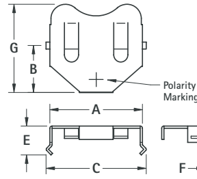
DWG. 2 - THRU HOLE MOUNT (THM) MATERIAL: .010 (.25) thick Phosphor Bronze, Tin Nickel Plate
