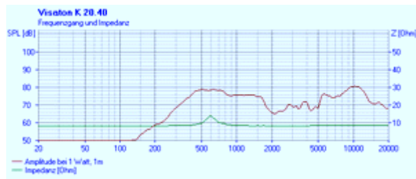
frequency- and impedance response
