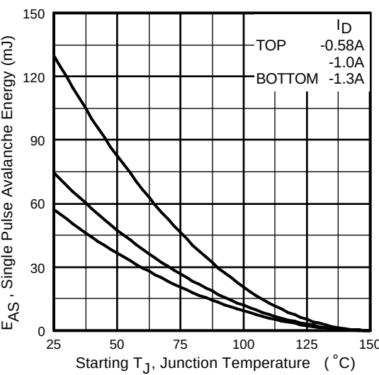
Fig 8. Maximum Avalanche Energy Vs. Drain Current
