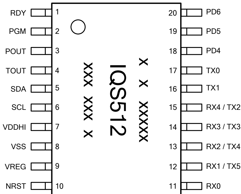
Figure 2.3 TSSOP Top View
