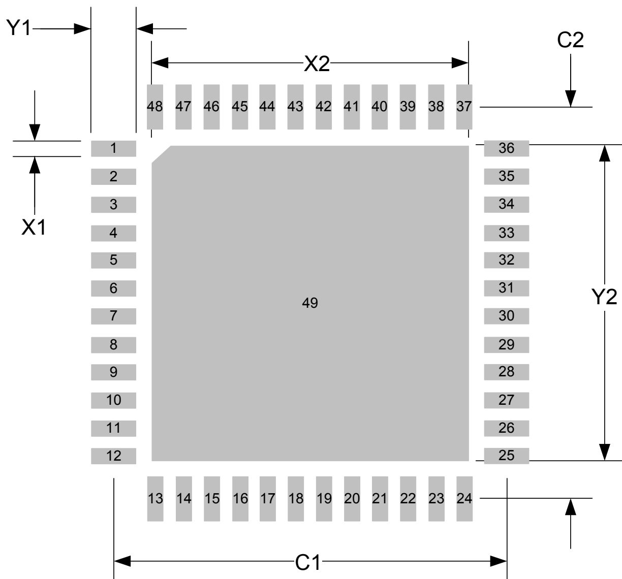
Figure 8.2 QFN(7x7)-48 Footprint
