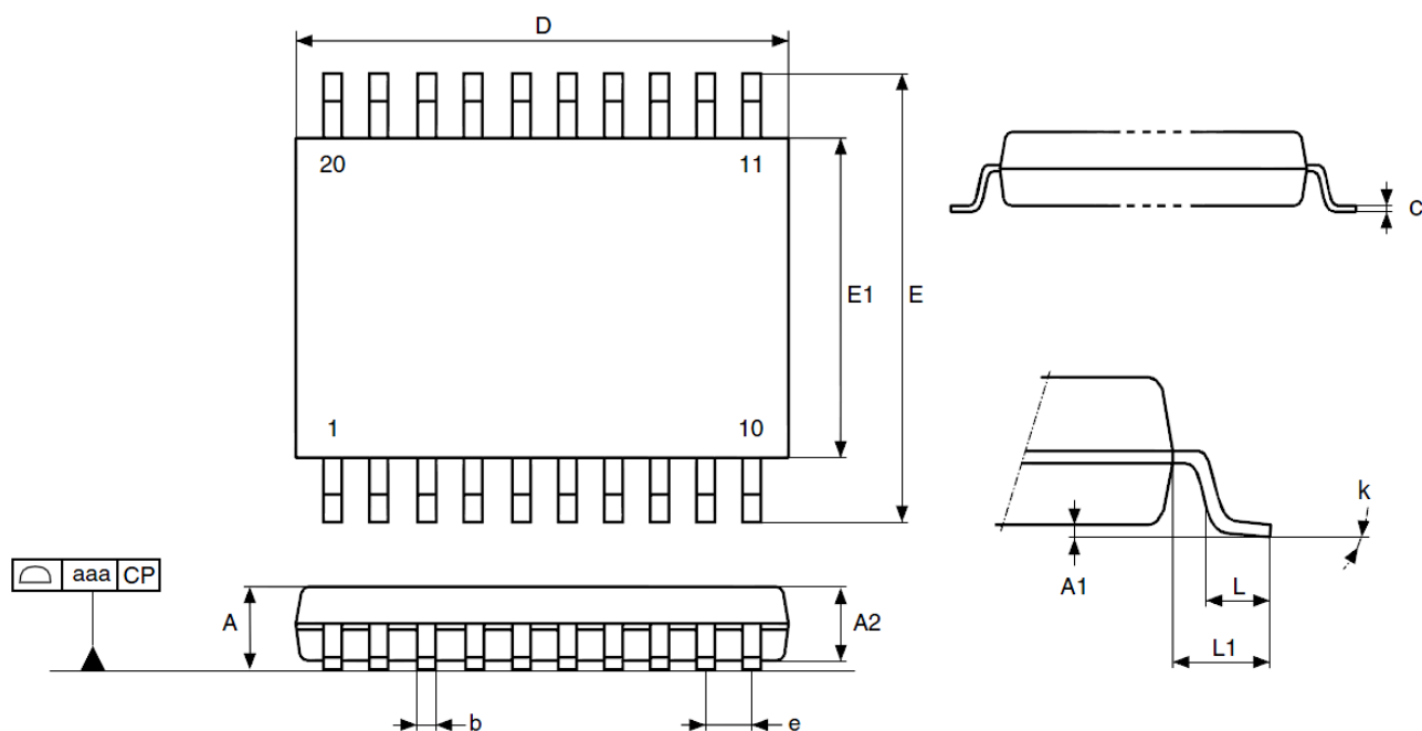
Figure 8.5 TSSOP20 Package
