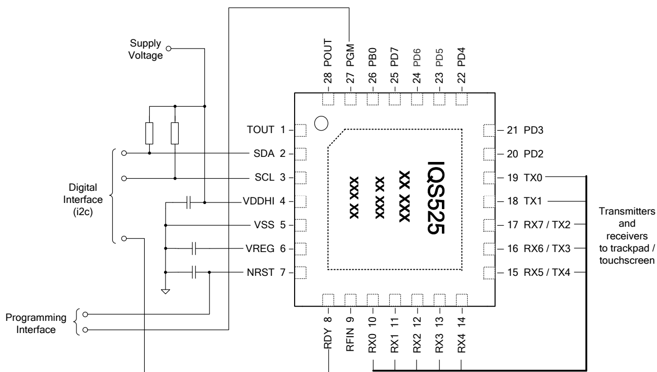
Figure 6.2 IQS525 Overview Diagram
