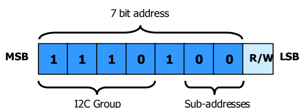
Figure 5.1 I 2 C Control Byte
