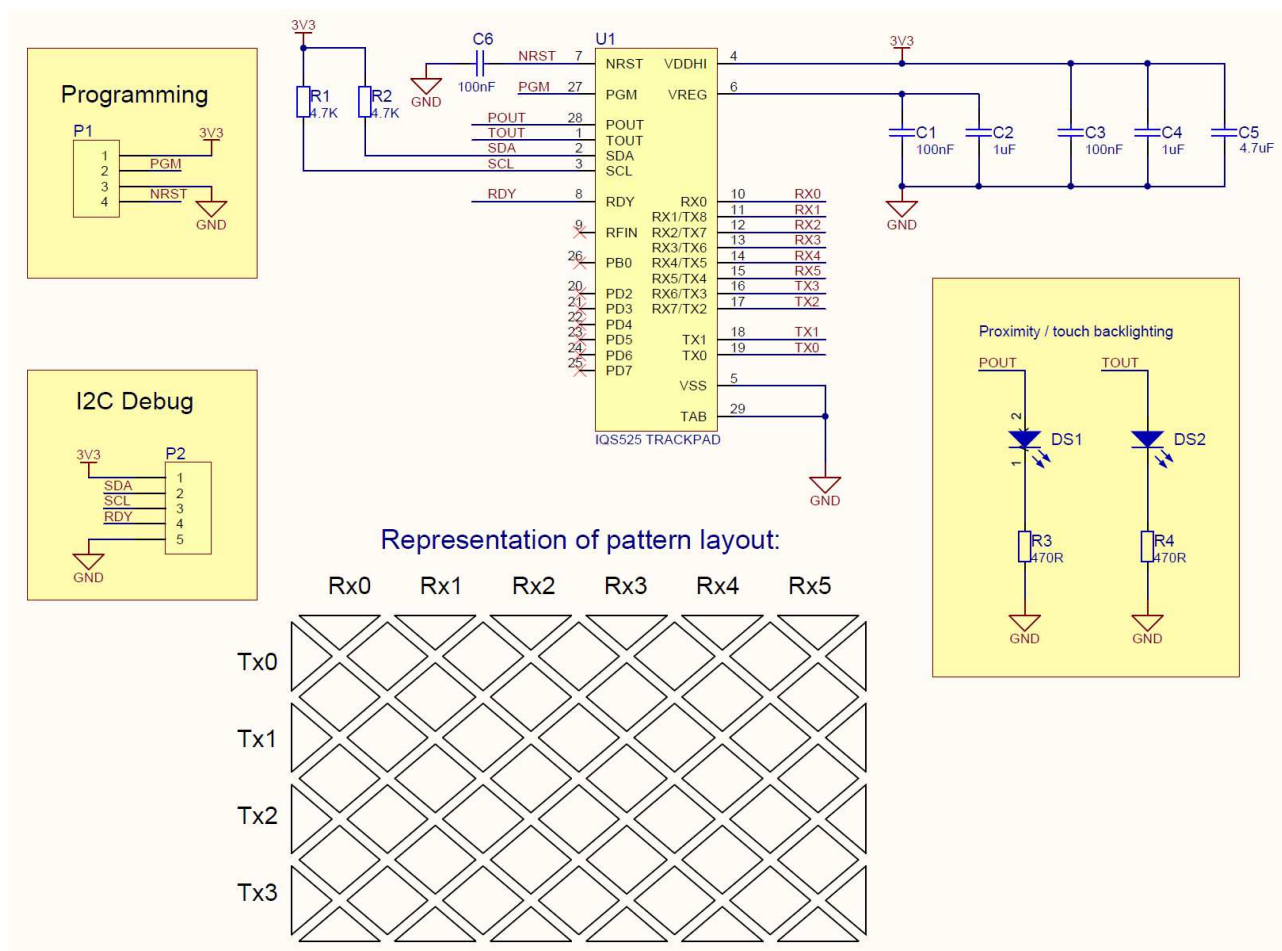
Figure 6.5 IQS525 Application Circuit
