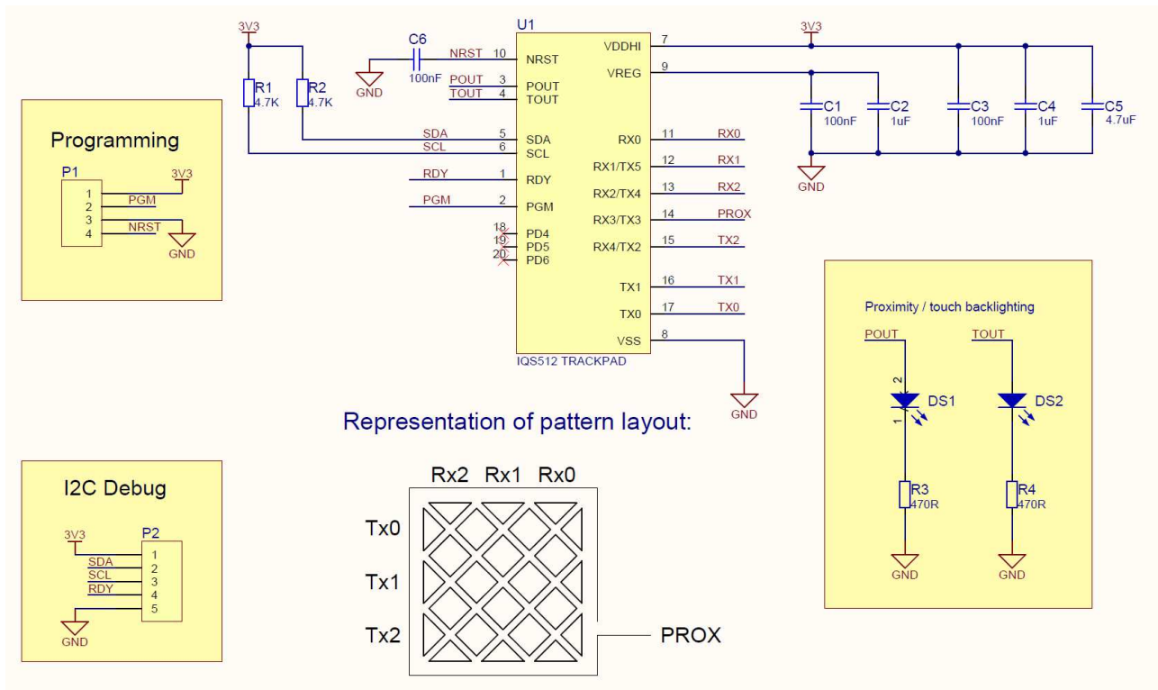
Figure 6.6 IQS512 Application Circuit
