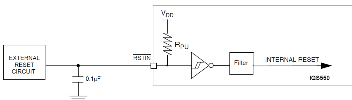
Figure 7.1 Recommended NRST pin configuration
