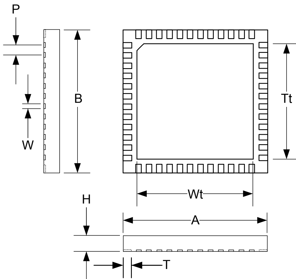
Figure 8.1 QFN(7x7)-48 Package
