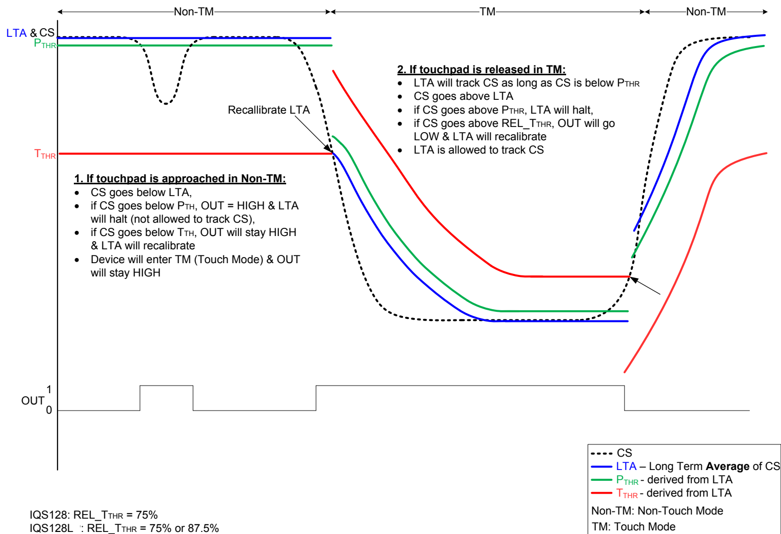
Figure 5.1 DYCAL Operation
