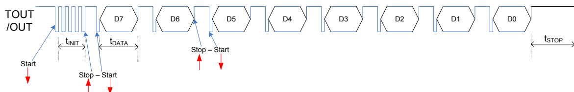
Figure 7.1 Debug: 1-wire streaming Debug Mode
