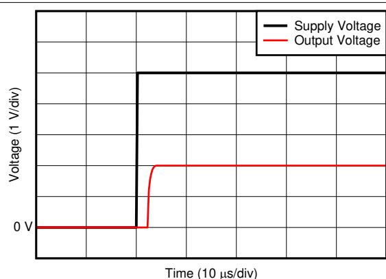
Figure 7-35. Start-Up Response
