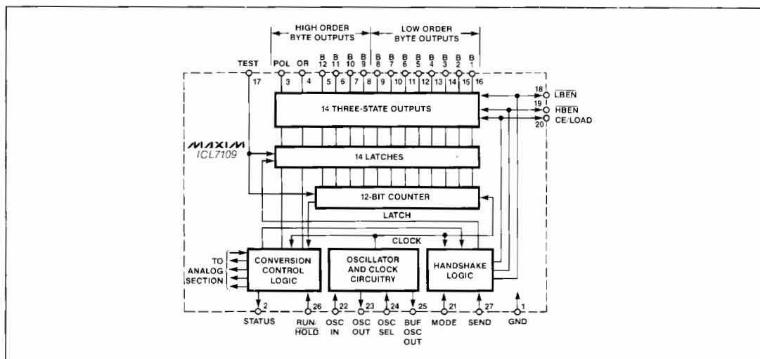
Figure 4. Digital Section
