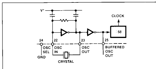
Figure 7. Crystal Oscillator
