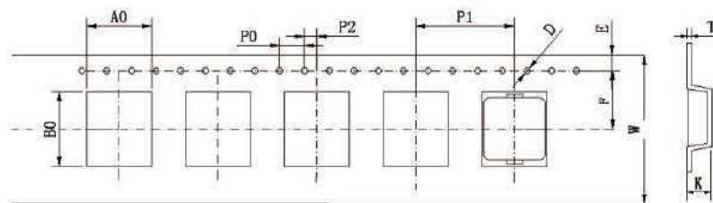
Tape Dimensions (mm)
