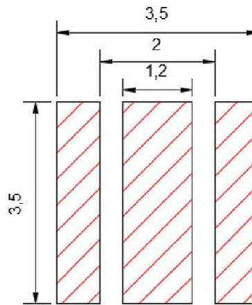
Recommended Soldering pad Layout (Unit: mm)
