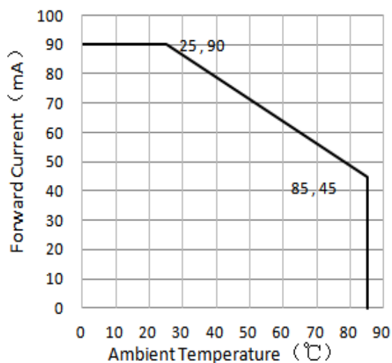
Ambient Temperature VS Allowable Forward Current 周围温度与允许电流特性
